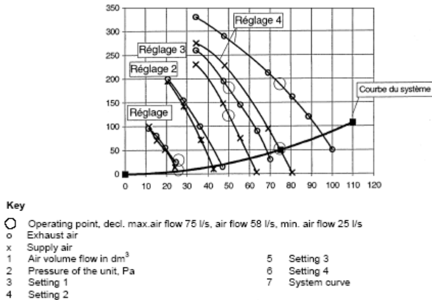
Figure 4-12: Characteristic line of products with heat recovery (here also with multi speed)
