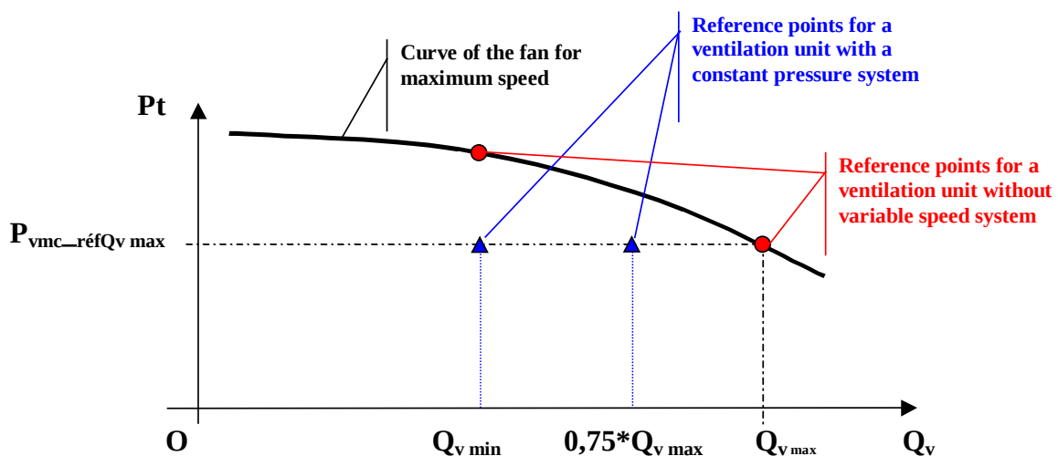
Figure 4-18: Running points chosen for a fan unit with constant pressure control system (Vialle &amp; al., 2007)
