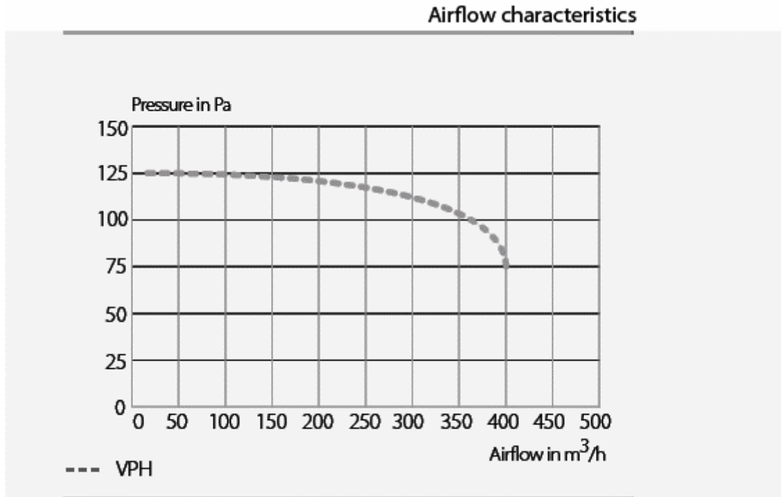
Figure 4-7: Characteristic line (Type b) of ICV product
