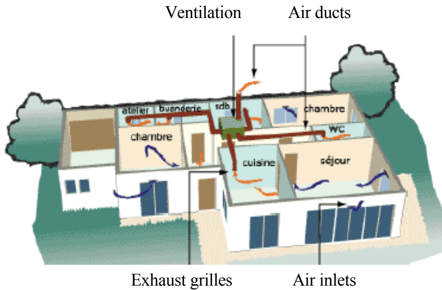
Figure 3-1: Centralized mechanical exhaust and natural supply ventilation system, from (ADEME, 2007)
