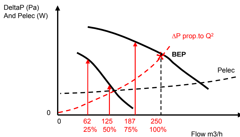
Figure 4-20: Typical ICV characteristic line and progression of testing to obtain EEI PL
