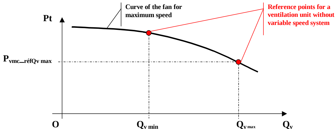
Figure 4-17: Running points chosen for a fan unit without control system (Vialle &amp; al., 2007)
